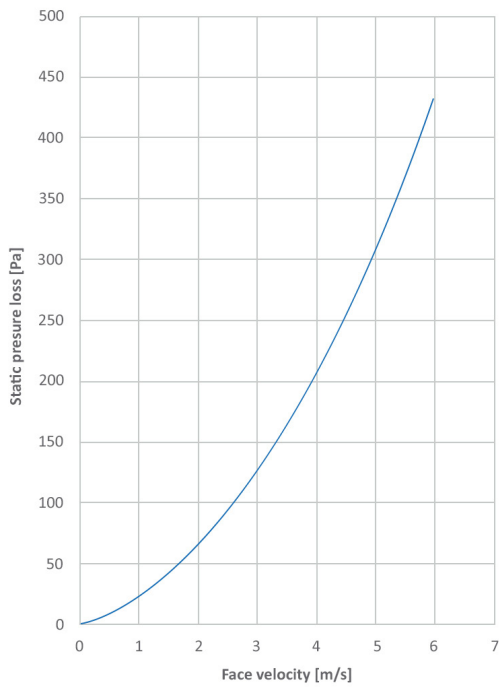
Initial pressure loss (Pa) for SE2 eliminator
