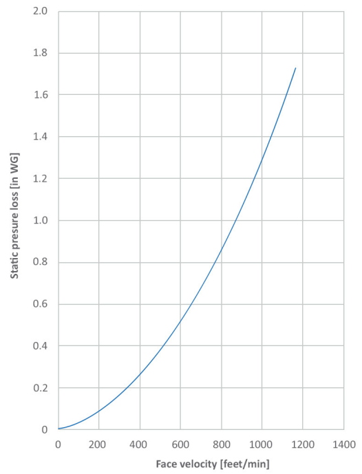
Initial pressure loss (in WG) for SE2 eliminator
