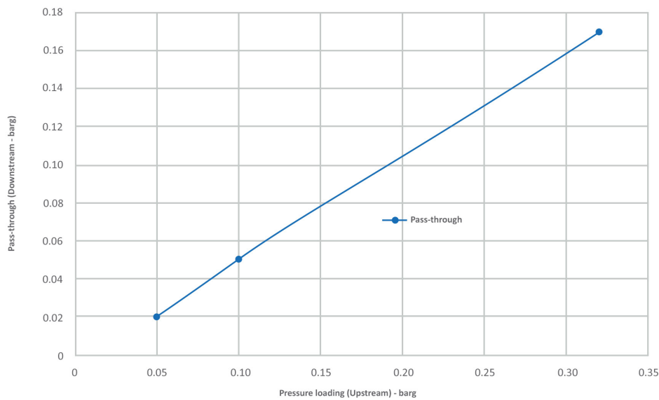
Long Duration Blast Testing
